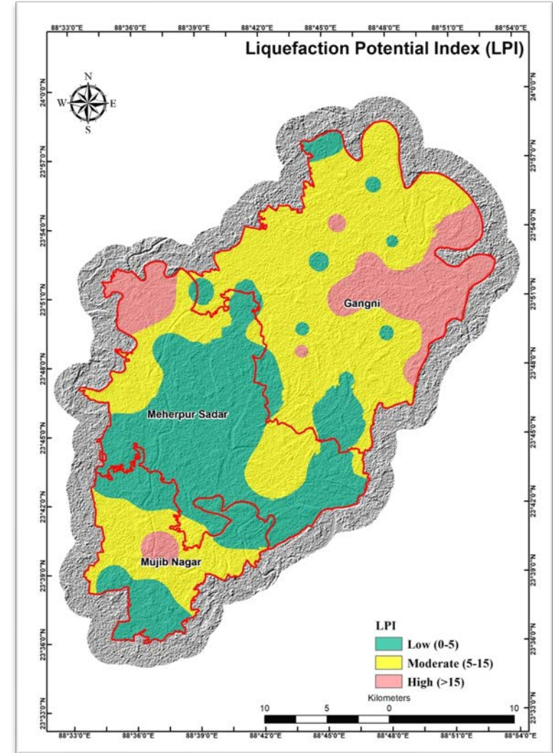
Liquefaction Potential Index Map
