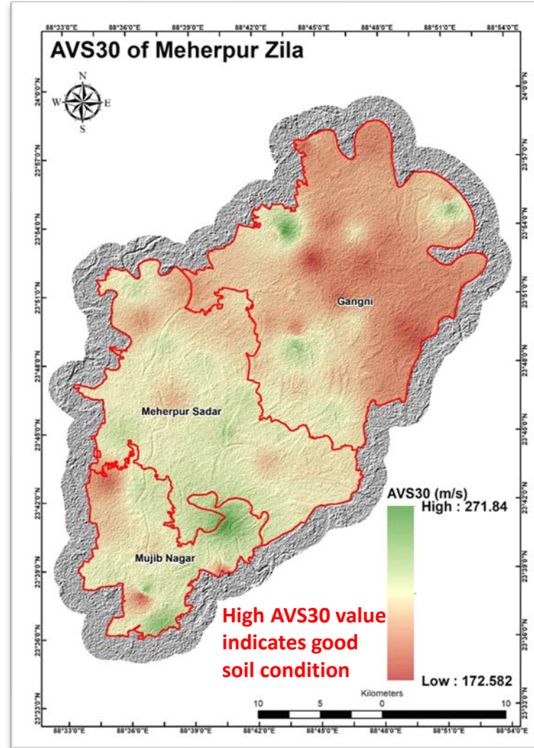
Engineering Geological Map
